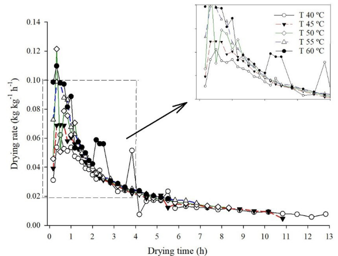
Figure 1. Drying rate of peanut seeds at different drying air temperatures.
