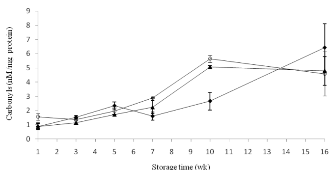
Figure 3. Protein carbonyl in chicken pâté during storage: (♦) T1, control (no additives); (▲) T2, nanoemulsion (6 % w/w); and (○) T3, BHT (100 mg/kg) and sodium nitrite (150 mg/kg).
