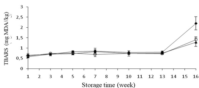
Figure 4. Values of peroxide index and TBARS during 16 weeks of refrigerated storage: (♦) T1, control (no additives); (▲) T2, nanoemulsion (6 % w/w); and (○) T3, BHT (100 mg/kg) and sodium nitrite (150 mg/kg).
