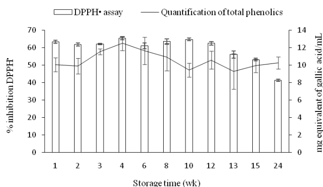
Figure 2. In vitro antioxidant activity of nanoemulsions encapsulating oregano essential oil over the storage period, expressed in % inhibition DPPH• and quantification of total phenolic content.
