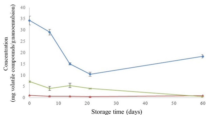
Figure 1. Temporal profiles of the concentration for (●) carvacrol, (■) \gamma -terpinene, and (▲) thymol during 60 days of refrigerated storage of OEO-NEs.
